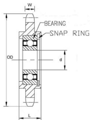
#80 and 100 Sprockets
