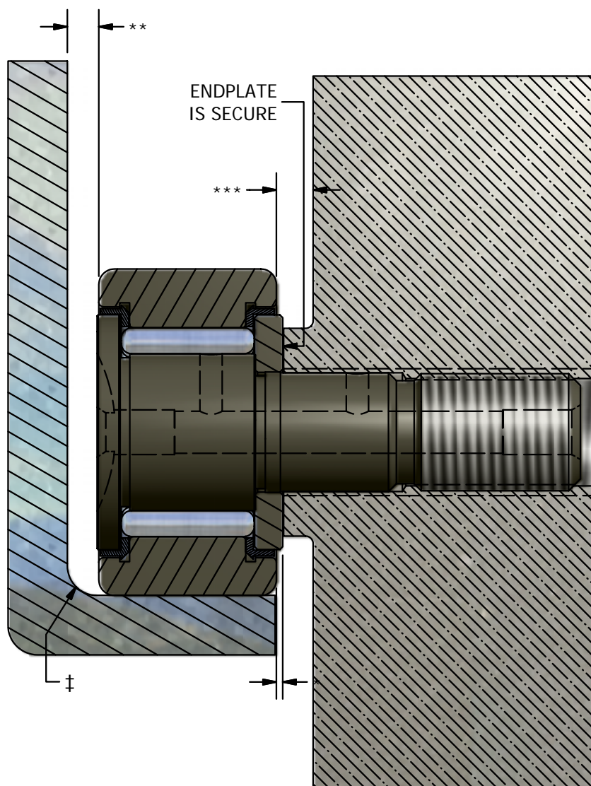
SECTION B-B SCALE 1.75
